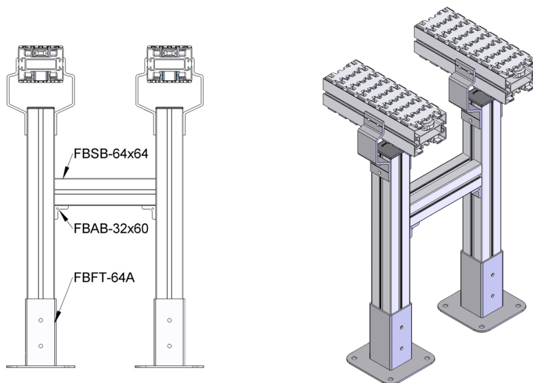
Double Support Structure FK, FS, FM, FC
