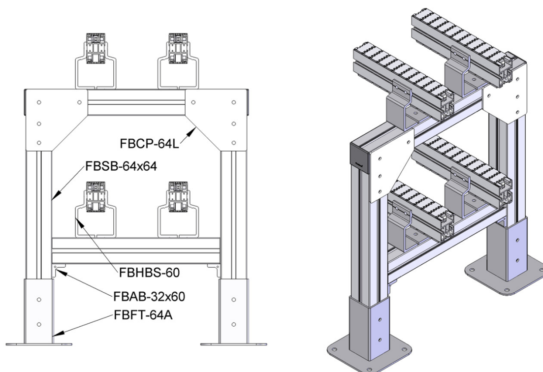
Multi Lane Double Layer Support Structure FK, FS, FM, FC, FL
