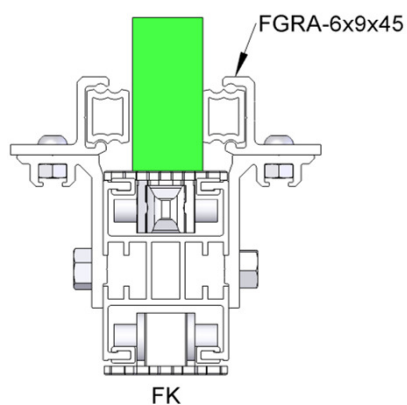
Small Box Guide Rail Assembly
