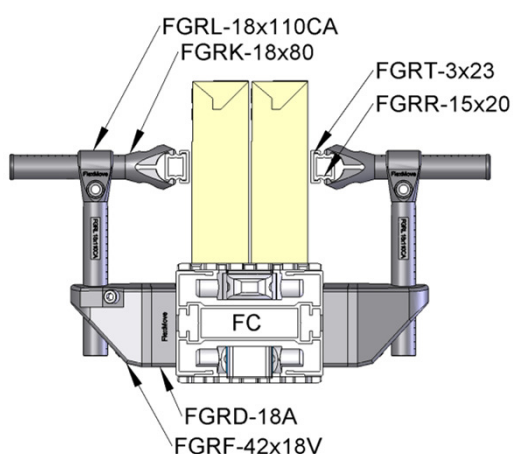
Width & Height Adjustable Guide Rail Assembly
