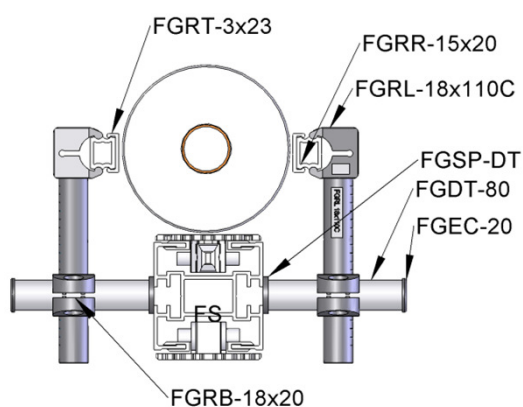
Width & Height Guide Rail Assembly
