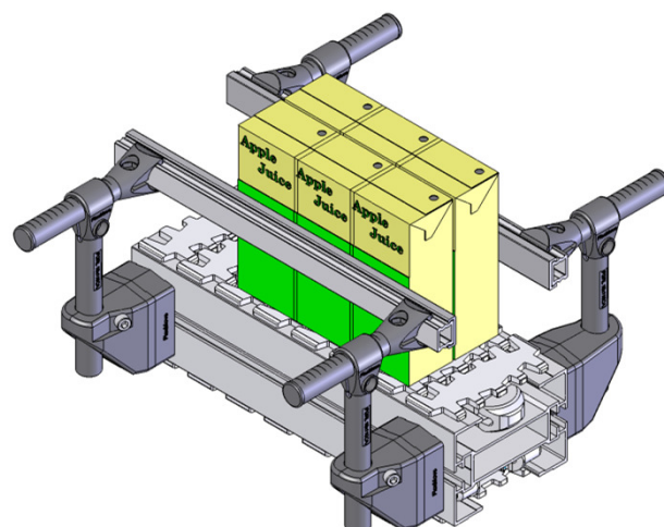
Box Handling
