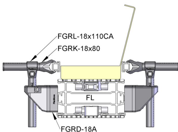
Width & Height Adjustable Guide Rail Assembly
