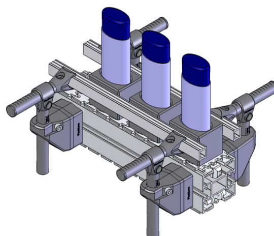
Pucks Handling
