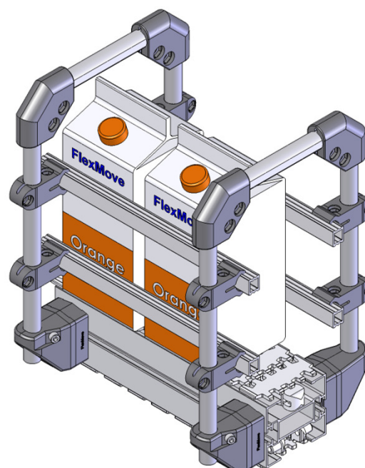
Box Handling
