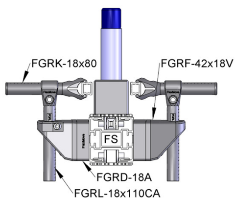
Width & Height Adjustable Guide Rail Assembly
