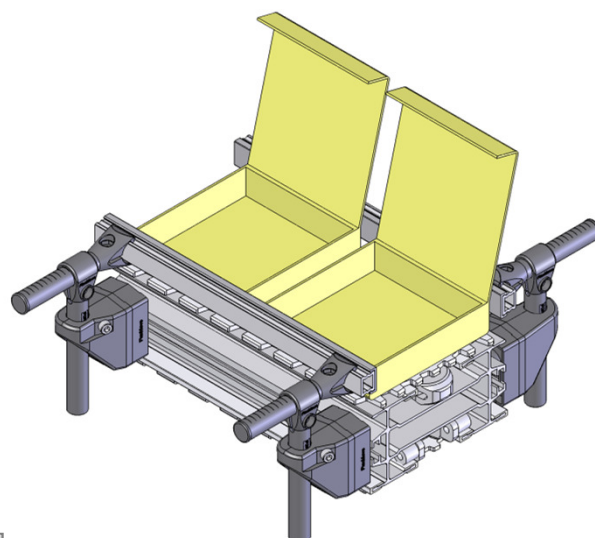
Packaging Box Handling
