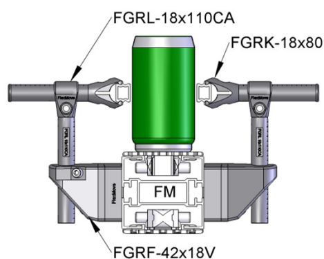
Width & Height Adjustable Guide Rail Assembly
