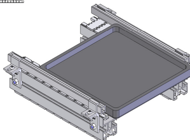
Pallet Handling
