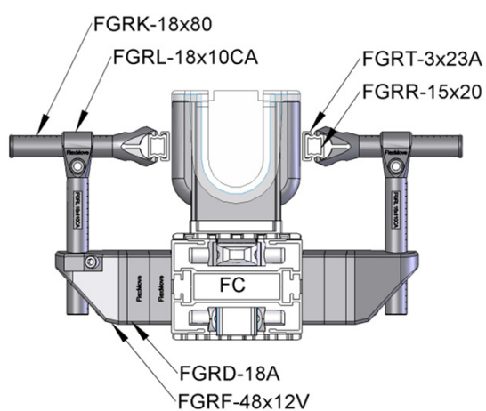
Pallet Assembly line Guide Rail
